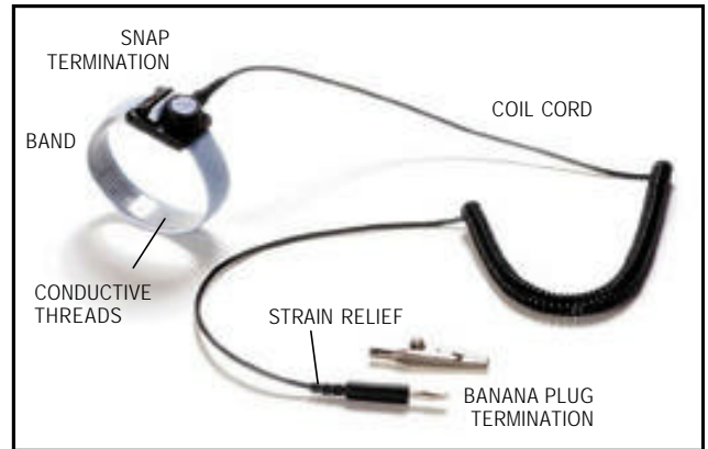
PHOTO 1. WRIST STRAP.
