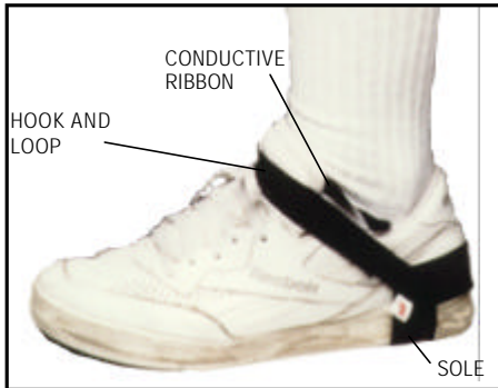
PHOTO 2. HEEL GROUNDER
